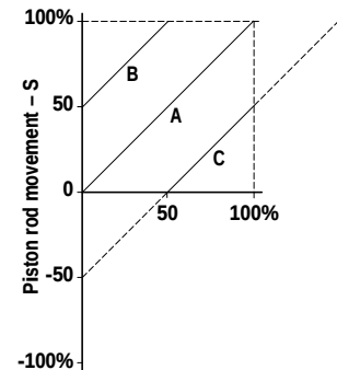
Figure 89: Zero adjustment graph
