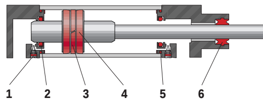
Figure 31: Types of seals
