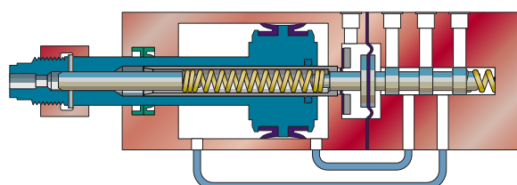
Figure 85: Fixed range positioner
