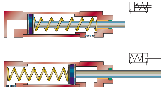
Figure 2: Single acting cylinder
