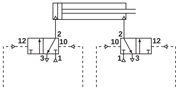
Figure 29: Pre-exhaust circuit
