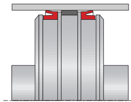
Figure 33: Section of a cup seal
