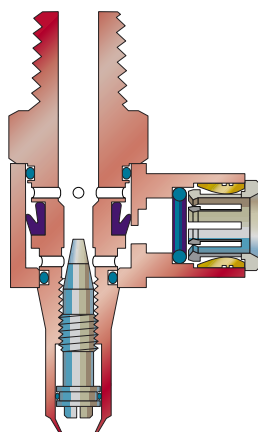
Figure 25: Banjo flow regs
