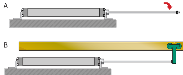
Figure 57: Long stroke
