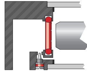
Figure 36: Cushion seal
