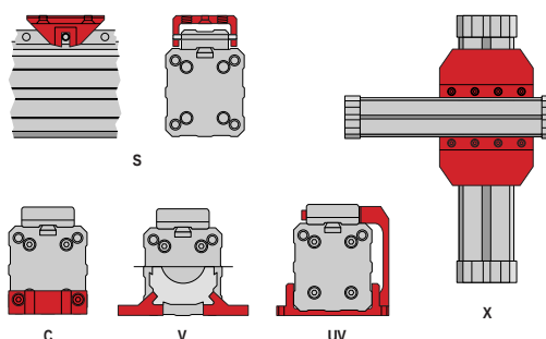
Figure 74: Rodless cylinder mountings
