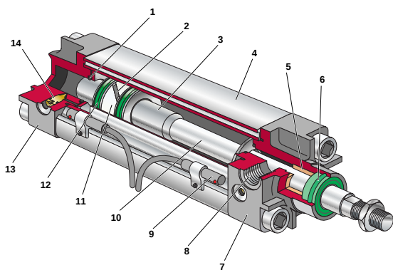
Figure 1: Main components of a cylinder
