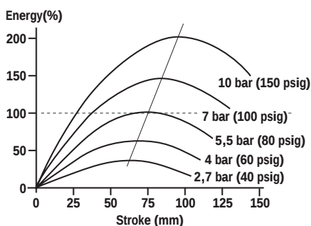
Figure 94: Energy graph
