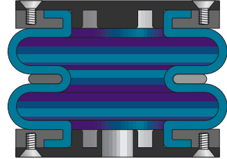
Figure 14: Bellows
