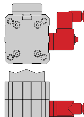
Figure 73: Integrated valve
