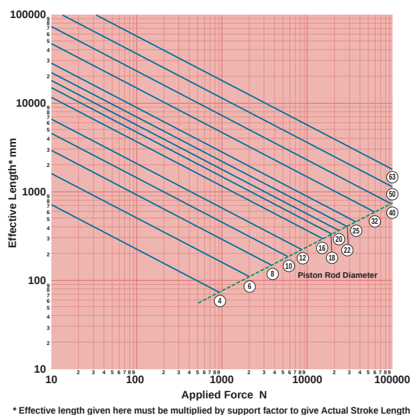
Figure 21: Maximum stroke length
