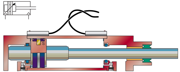
Figure 7: Magnetic cylinder
