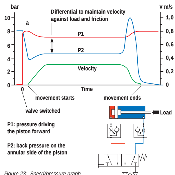
Figure 23: Speed/pressure graph
