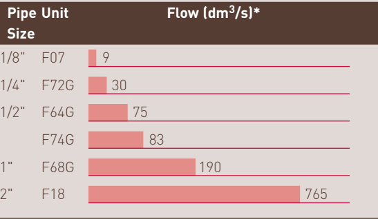
Figure 10. GENERAL PURPOSE FILTER FLOWS
