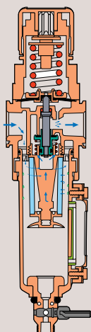
Figure 18. General Purpose Filter/Regulator
