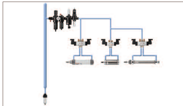
Figure 26. Shut-off valve, filter/reg, Micro-Fog lubricator, soft start/dump, relief valve.
