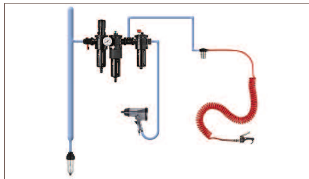
Figure 27. Shut-off valve, filter/regulator, oil removal filter, porting block, Micro-Fog lubricator.
