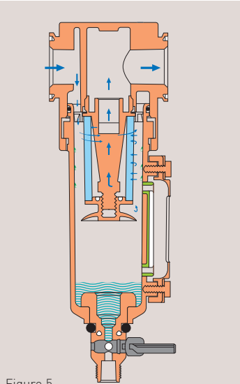
Figure 5. General Purpose Filter
