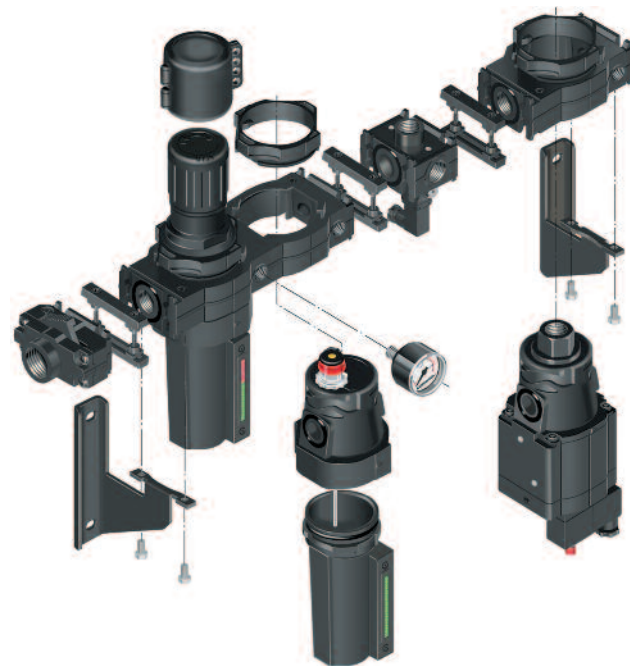
Figure 34. Olympian Plus System - Typical elements and features of a modular system.
