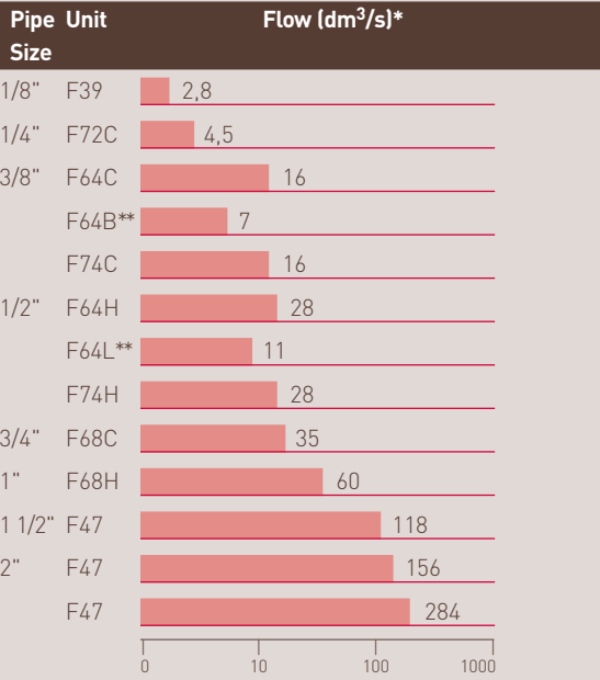
Figure 11. HIGH EFFICIENCY FILTER FLOWS
