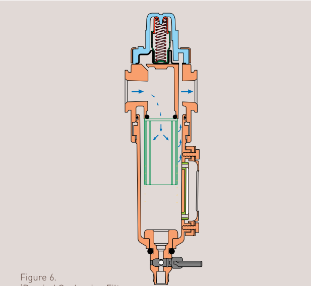
Figure 6. 'Puraire' Coalescing Filter
