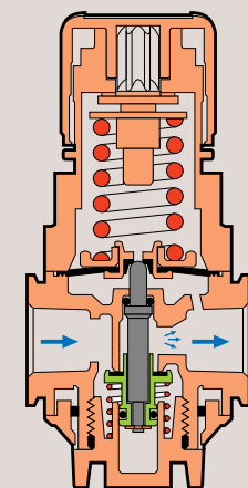
Figure 13. General Purpose Regulator
