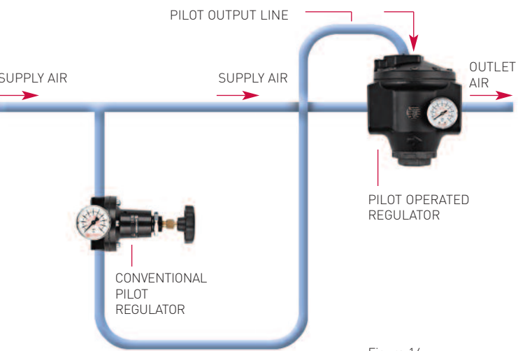
Figure 14. A typical pilot operated regulator installation.
