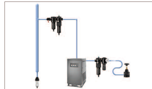
Figure 31. Shut-off valve, general purpose filter, oil removal filter, dryer, oil removal filter, regulator and precision regulator.
