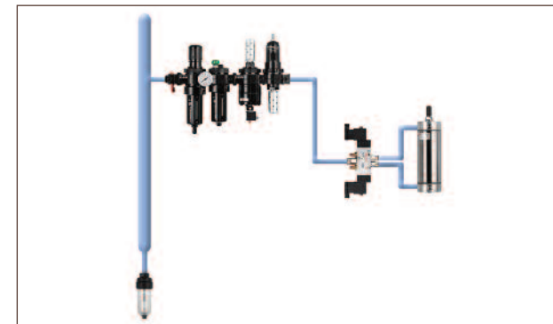
Figure 30. Shut-off valve, filter/reg, Oil-Fog lubricator, soft start/dump valve, relief valve.
