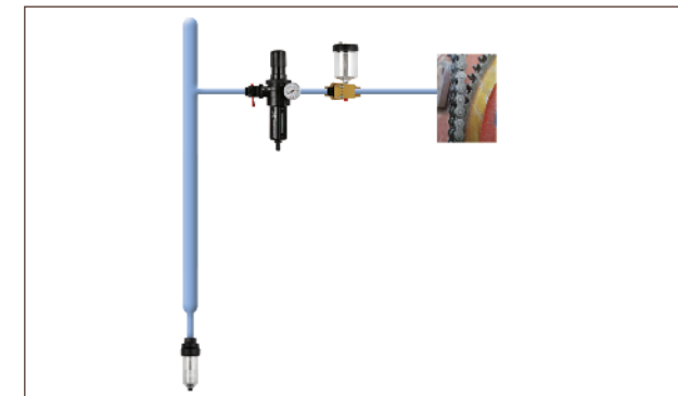
Figure 32. Shut-off valve, filter/reg + direct injection lubricator.
