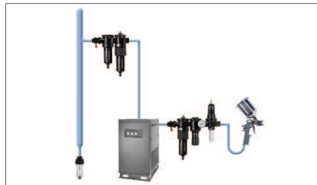
Figure 29. Shut-off valve, general purpose filter, oil removal filter, dryer, oil removal filter, regulator, relief valve.
