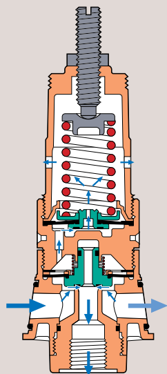
Figure 23. Internal Pilot Relief Valve
