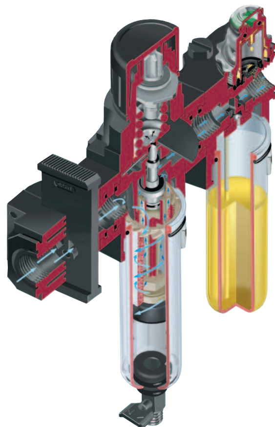
Figure 33. Excelon System - Typical workings of an air preparation assembly.
